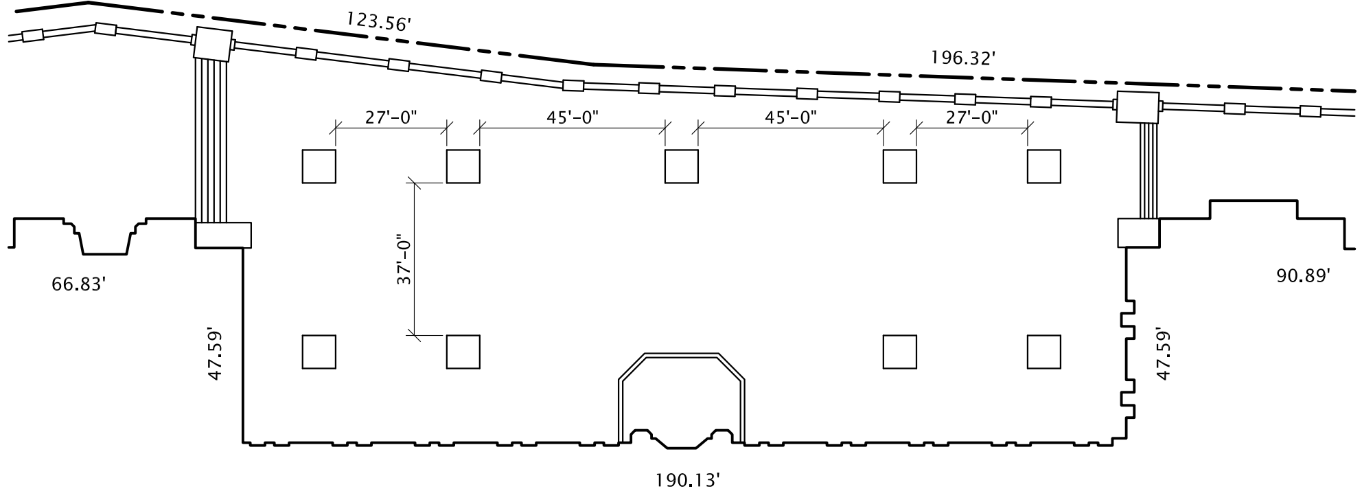
1 EAST PLAZA PLAN 1/32" = 1'-0" N
